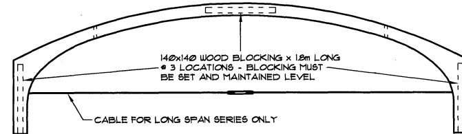
BLOCKING FOR STORAGE PLAN VIEW
