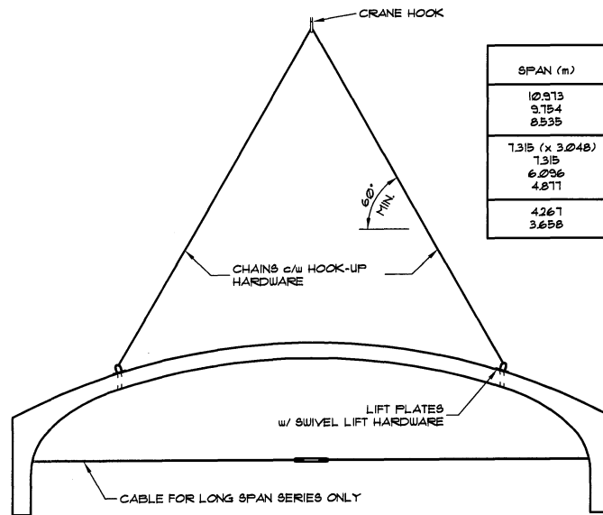
ARRANGEMENT FOR INSTALLATION ELEVATION VIEW
