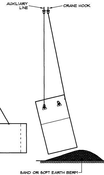
ARRANGEMENT FOR FLIPPING ELEVATION VIEW
