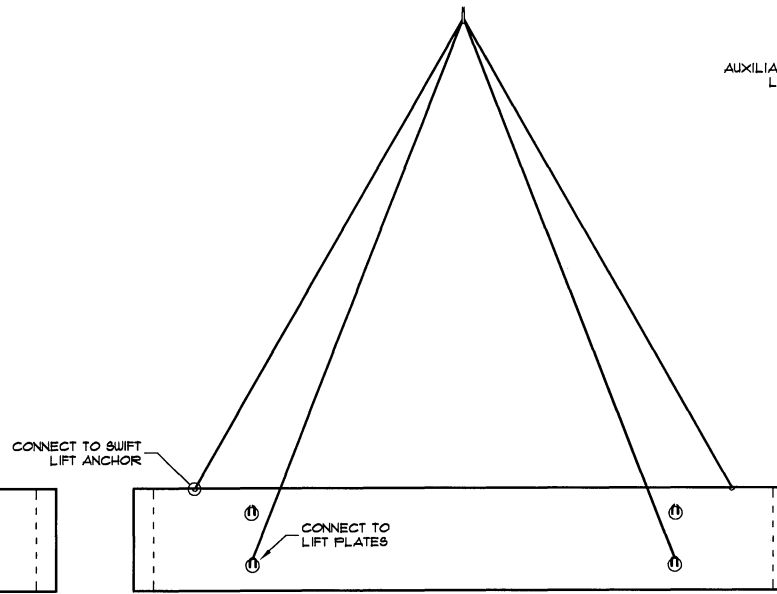
ARRANGEMENT FOR FLIPPING ELEVATION VIEW
