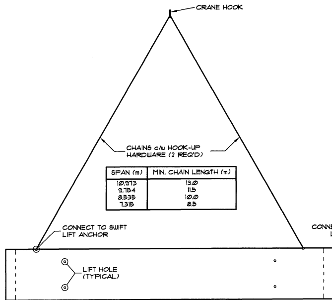
ARRANGEMENT FOR OFF-LOADING ELEVATION VIEW
