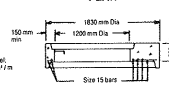
SECTION A-A TRANSITION SLAB
