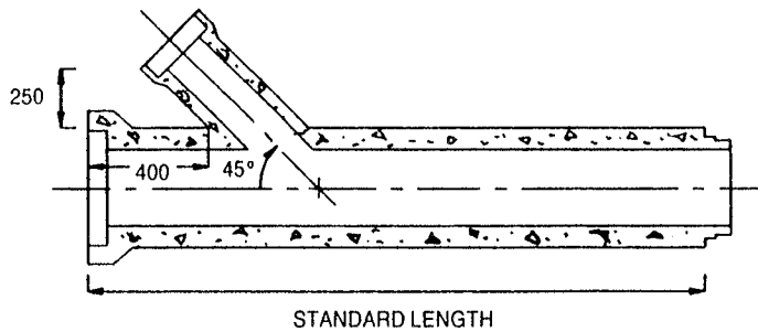
STANDARD WYE
