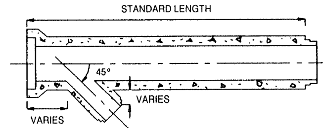
DROP WYE
