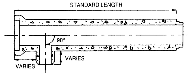
DROP TEE
