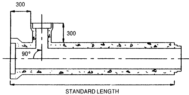
STANDARD TEE
