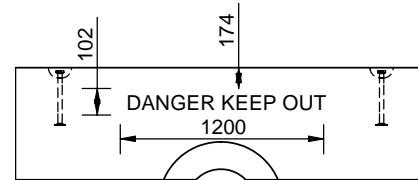
EMBOSSING DETAIL ON VERTICAL FACE
