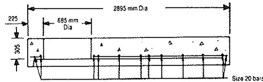
SECTION A-A FLAT CAP
