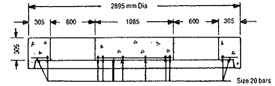
SECTION A-A TWIN INLET FLAT CAP
