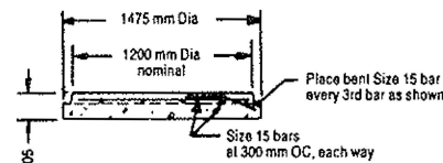
SECTION A-A BASE SLAB
