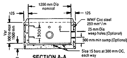
SECTION A-A MONOLITHIC BASE
