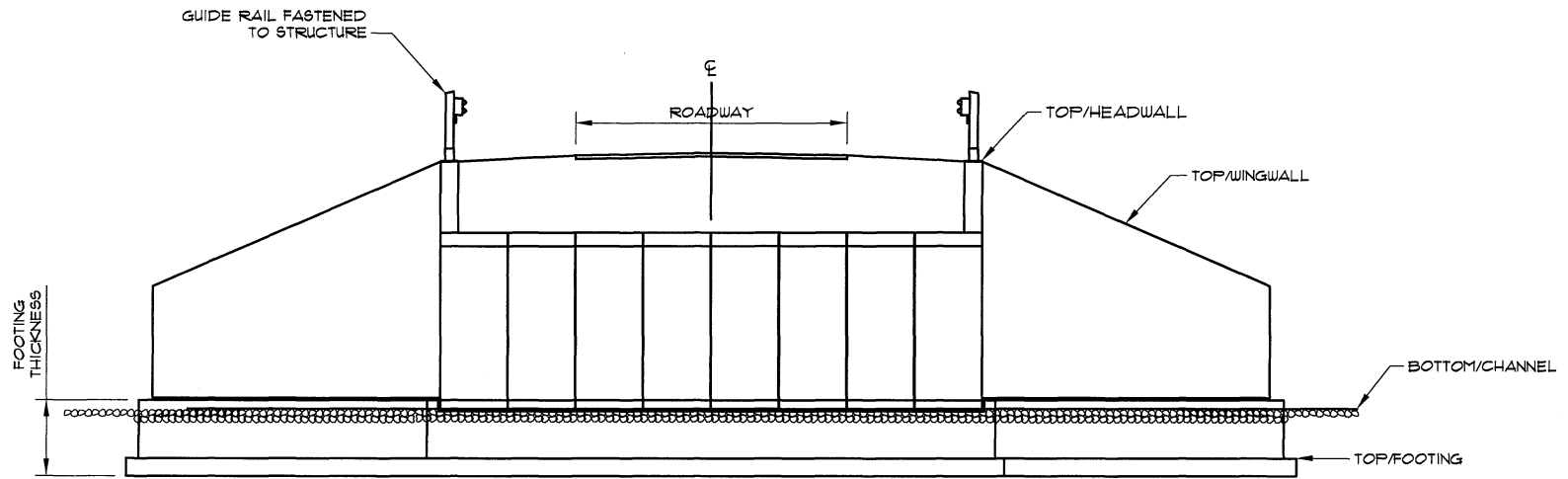
CULVERT PROFILE - OPTION 'A'
