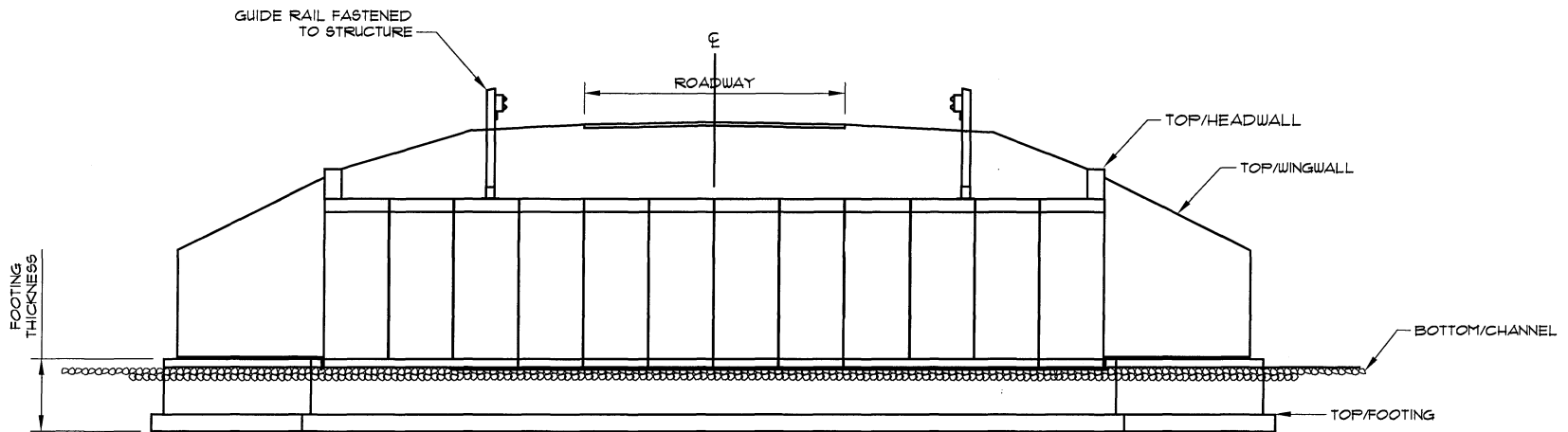
CULVERT PROFILE - OPTION 'B'
