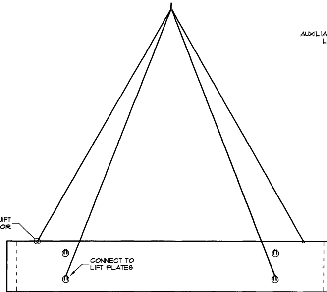
ARRANGEMENT FOR FLIPPING ELEVATION VIEW
