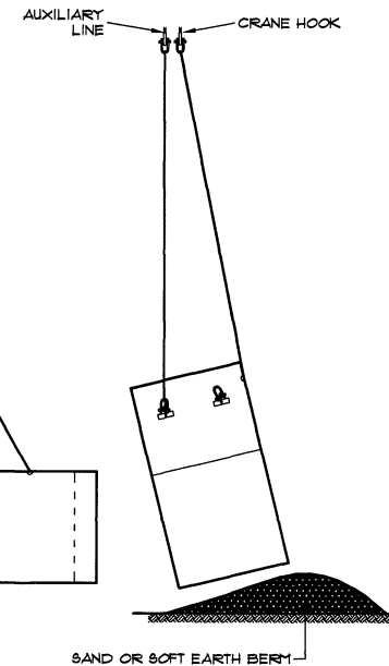
ARRANGEMENT FOR FLIPPING ELEVATION VIEW
