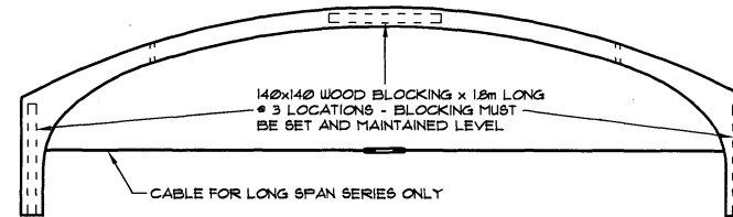
BLOCKING FOR STORAGE PLAN VIEW
